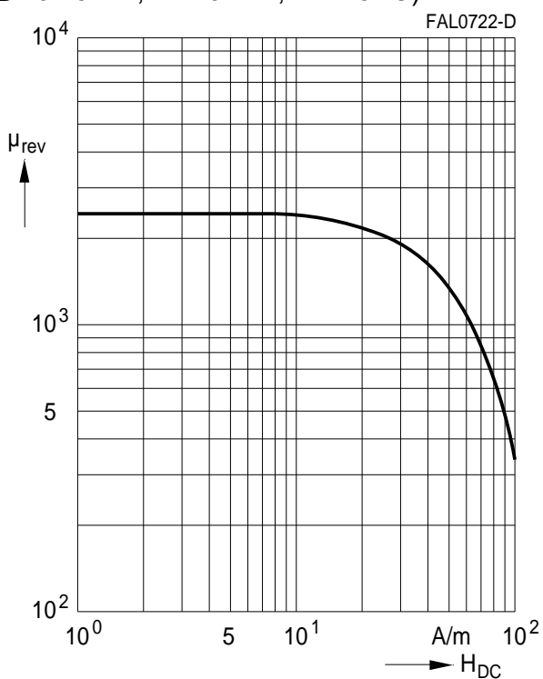
DC magnetic bias of RM cores (typical values) ( \hat{B} \leq 0.25 \text{ mT} , f = 10 \text{ kHz} , T = 25 \text{ }^\circ\text{C} )
